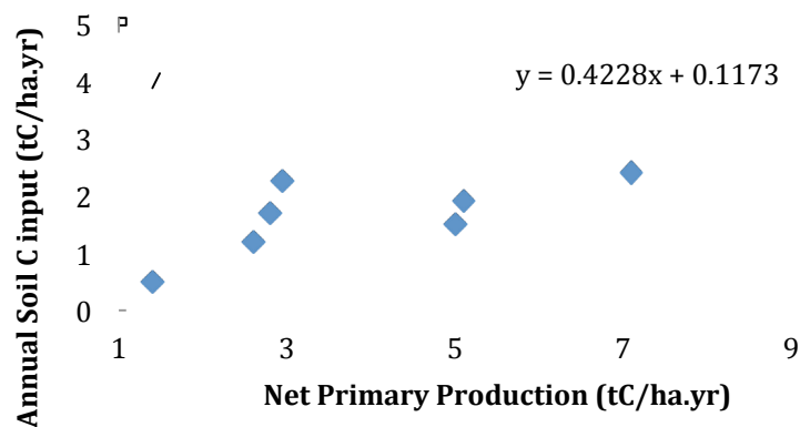
Figure 9. Carbon sequestration in soil is correlated with net primary productivity, a measure of photosynthetic C acquisition from the atmosphere.
